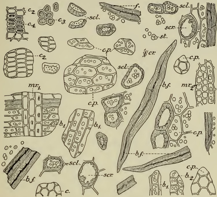
FIG. 100.—Powdered Cassia Bark. b 1 , b 2 , bast parenchyma in surface view and in section; b f , bast fibres; c 1 , c 2 , cork in surface view and in section; c 3 , c 4 , thick-walled cork in surface view and in section; c p , cortical parenchyma; cr , crystals of calcium oxalate; mr 1 , mr 2 , medullary ray in radial and in tangential section, with crystals of calcium oxalate; scl , sclerenchymatous cells; scr , secretion cells; st , starch. (Partly after Greenish and Collin.) ×150.
